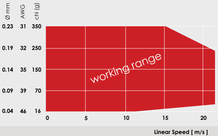
Wire / Tension
